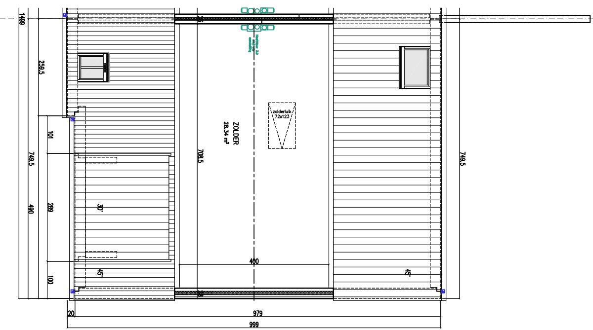
-woning Lot 5- -ZOLDERPLAN-
