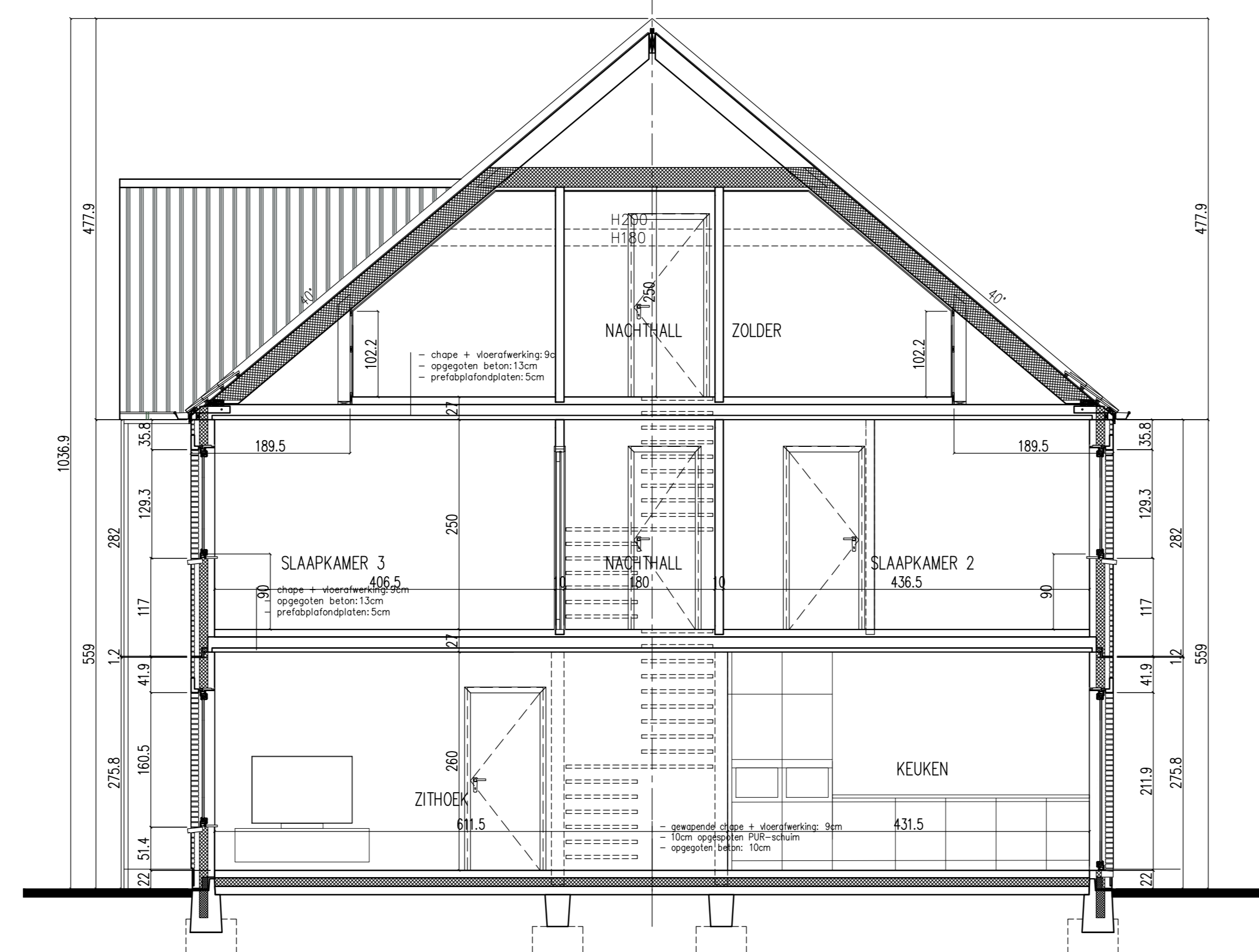
-DOORSNEDE AA- Lot 4
