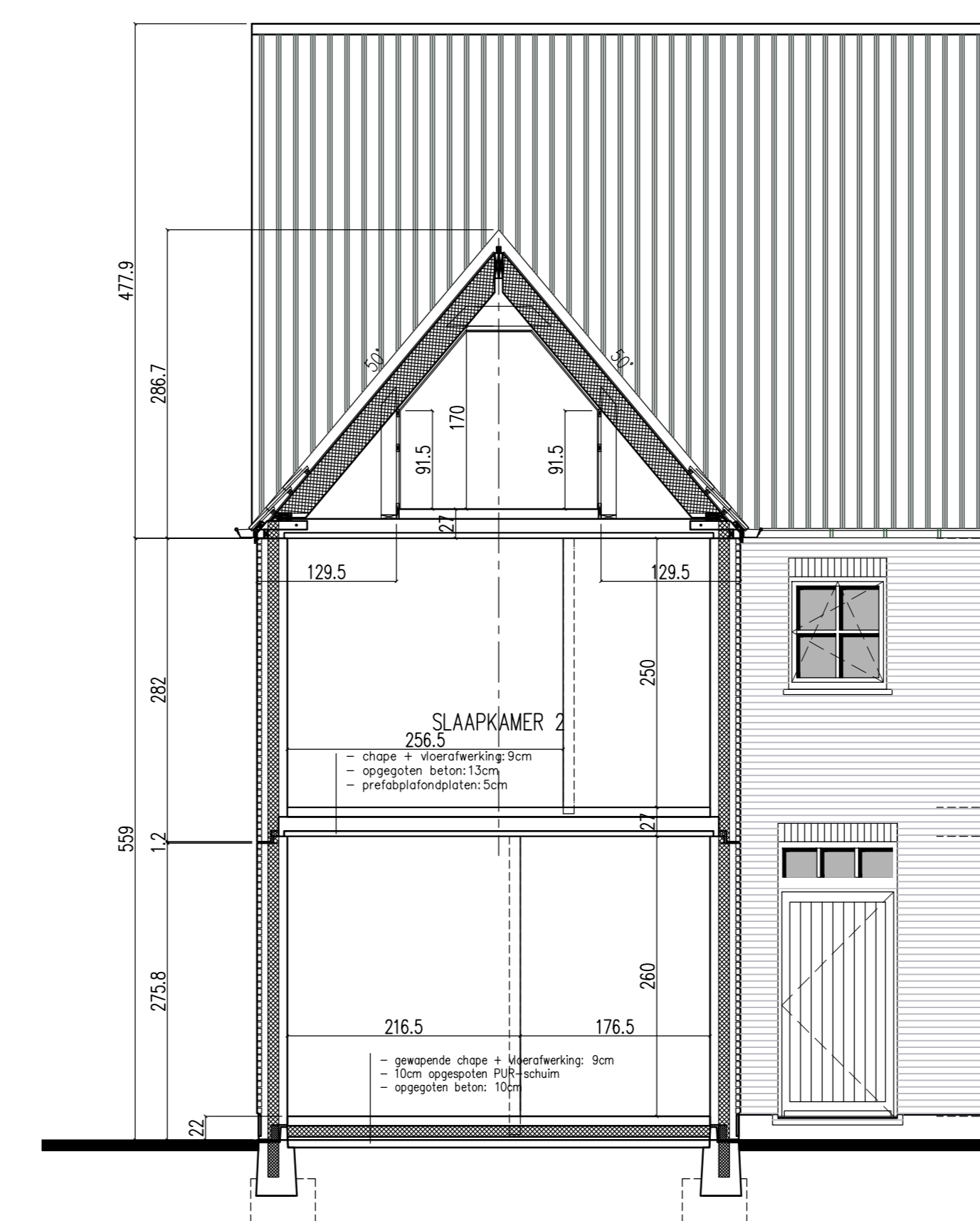
-DOORSNEDE BB- Lot 3
