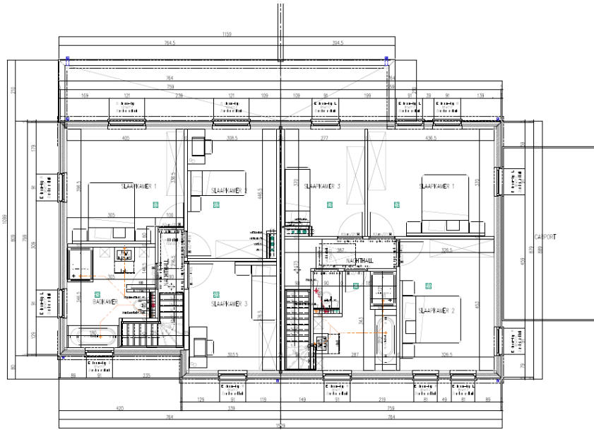
-VERDIEPING- (64,60m 2 ) B13242 - Lot 4
